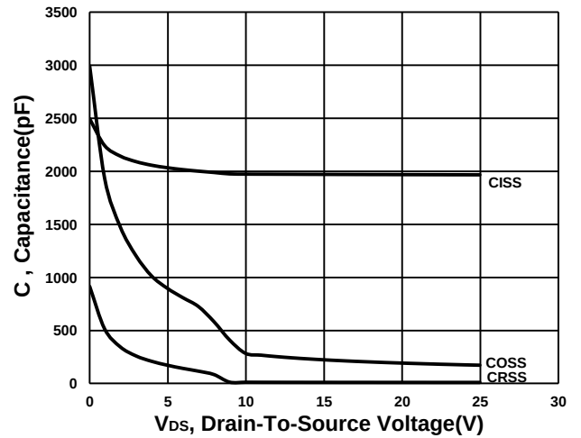
Capacitance Characteristic
